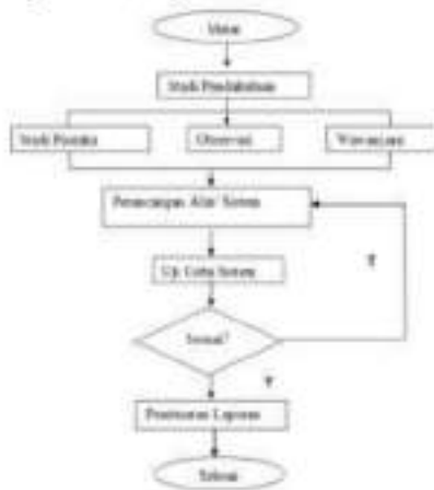
Gambar 1. Flowchar Penelitian
