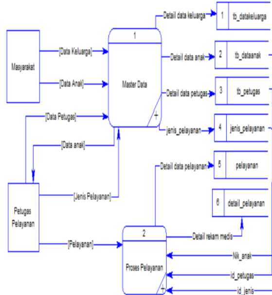
Gambar 5. DFD Level 1
