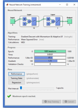
Figure 5 Implementation of Backpropagation Architecture
