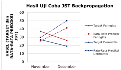
Figure 9 Average Trial Results Against Pharyngitis and Dermatitis Targets in November and December 2020
