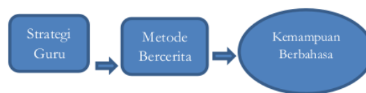
Gambar 1. Alur Penelitian
