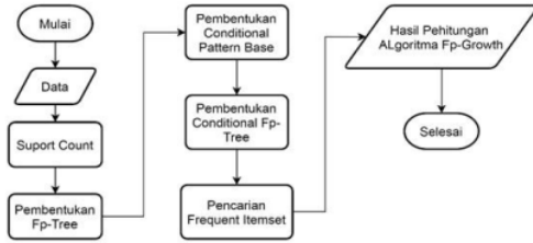
Gambar 1. Flowchart FP-Growth
