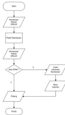
Gambar 4. Flowchart Sistem parkir lama
