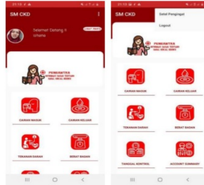
Gambar 6. Menu Dashboard
