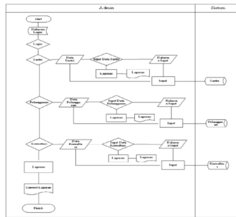
Gambar 2. Desain Flowchart
