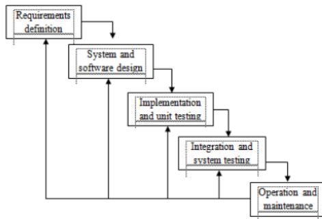
Gambar 1. Metode Waterfall
