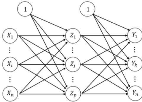
Figure 3. Architecture of Backpropagation
