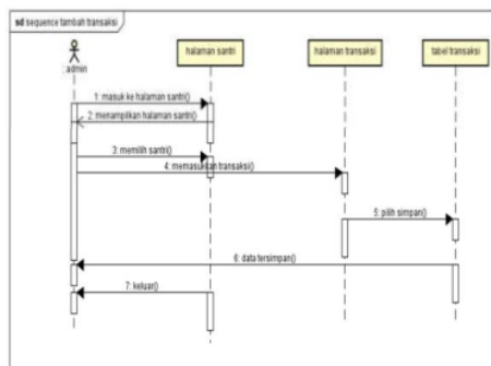
Gambar 4.7 sequence diagram tambah transaksi
