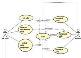
Gambar 4.1. Use case dompet santri
