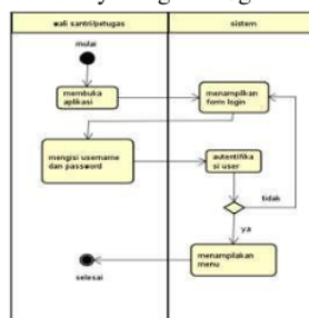
Gambar 4.2. activity diagram login.
