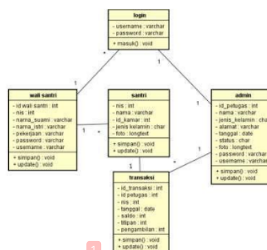
Gambar 4.8. Class Diagram
