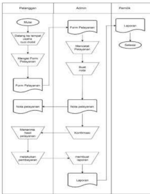
Gambar 1. Flowchart Sistem Kerja Eksisting
