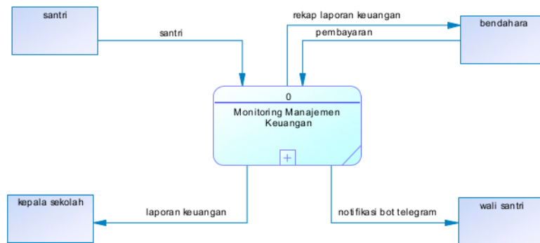
Gambar 2. Diagram Context
