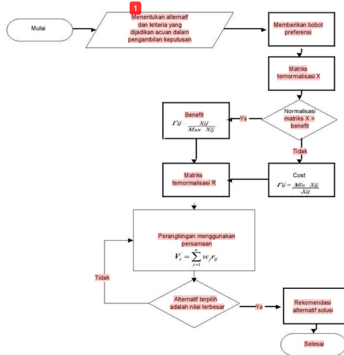
Gambar 3. Konsep Algoritma Simple Additive Weighting (SAW)
