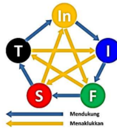
Figure 1: STIFIn Circulation Theory (Poniman & Hadiyat, 2015)
