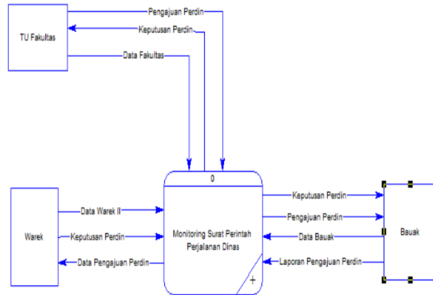
Gambar 5. Data Flow Diagram
