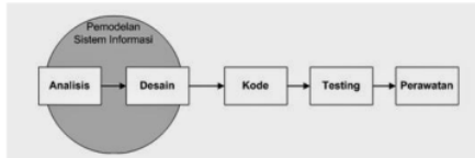
Gambar 1. Model Waterfall
