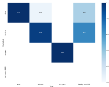
Gambar 15. Confusion Matrix Val
