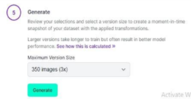
Gambar 9. Generate
