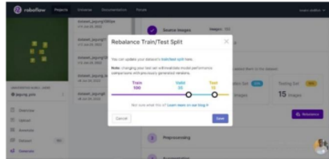
Gambar 8. Split Dataset
