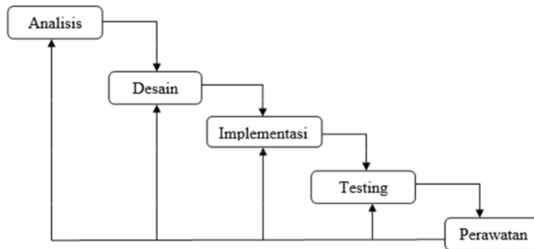
Gambar 1. Model Waterfall [10]
