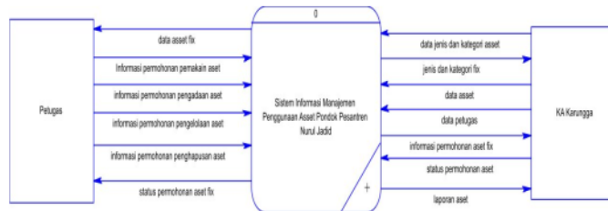
Gambar 4. Context Diagram
