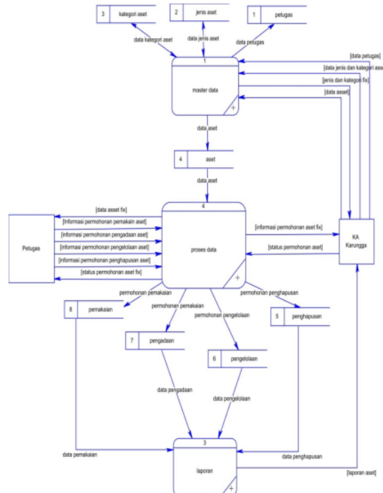
Gambar 5. Diagram Level 1
