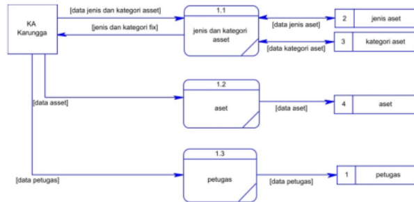
Gambar 6. DFD Level 2 Data Master
