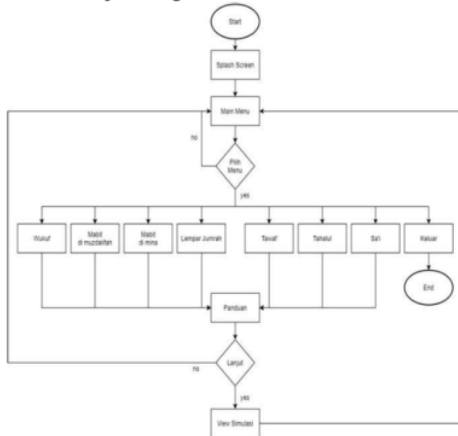
Gambar 4. Flowchat Virtual Reality Manasik Haji
