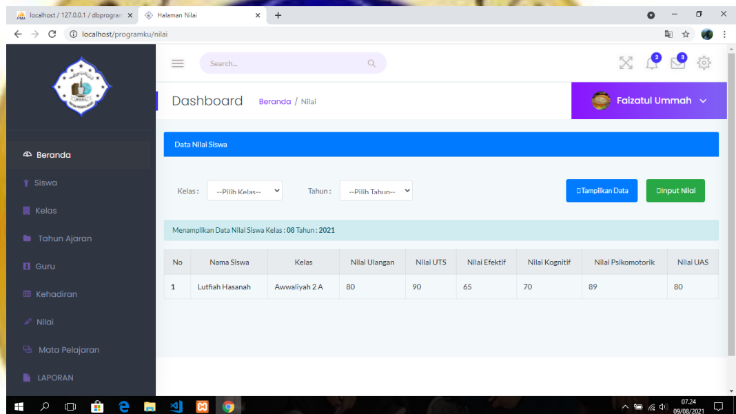
Gambar 4.33 Halaman Nilai
