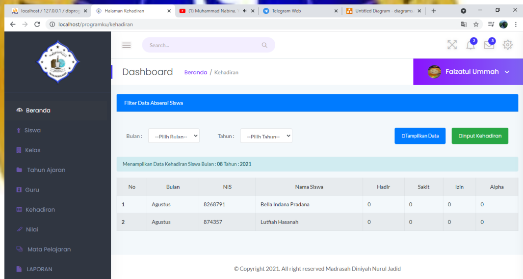
Gambar 4.31 Halaman Absen
