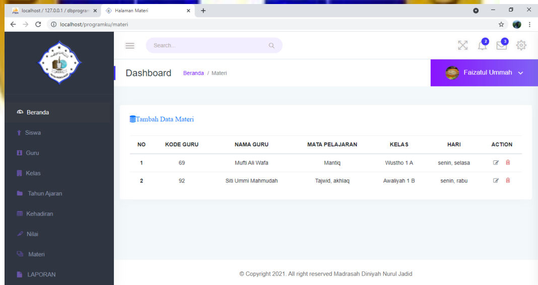
Gambar 4.35 Halaman Materi
