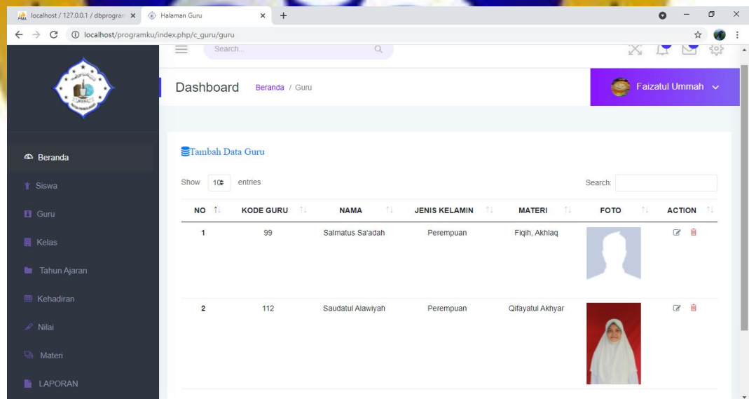
Gambar 4.25 Halaman Guru
