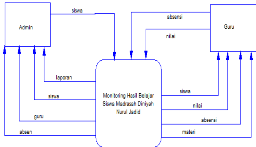
Gambar 4.3 Diagram Konteks
