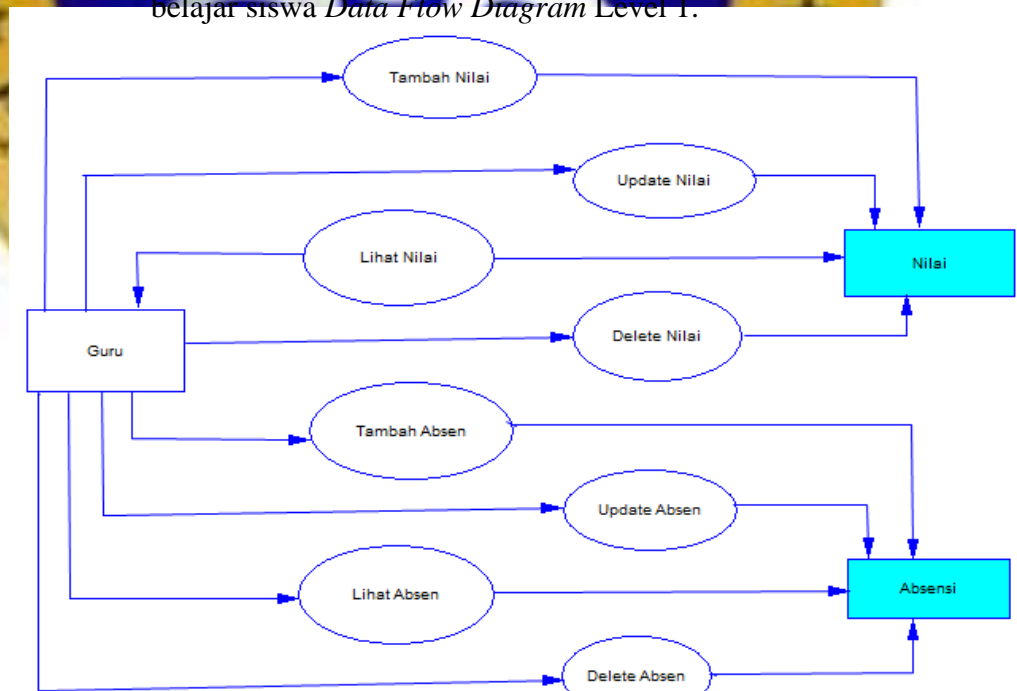
Gambar 4.7 DFD Level 2 Proses Laporan
