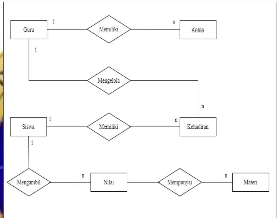
Gambar 4.8 Entity Relation Diagram (ERD)
