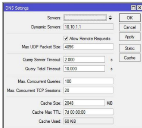
Gambar 4. Setting ip DNS
