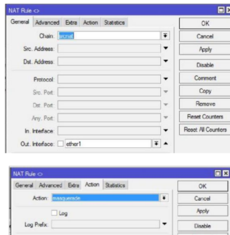
Gambar 5. Setting ip firewall NAT
