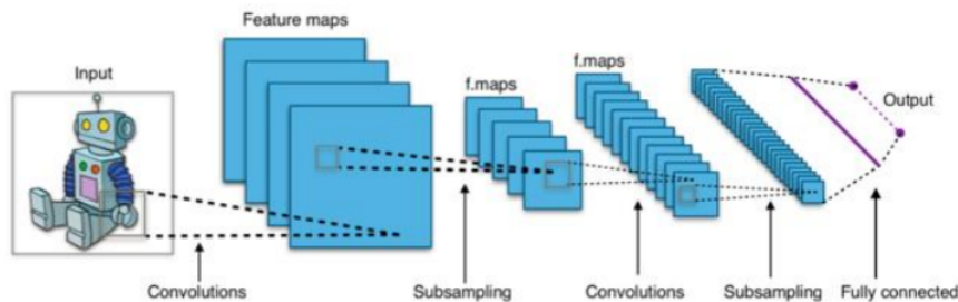
Gambar 1. Arsitektur Convolutional Neural Network (CNN)
